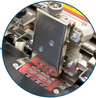
Rotating Air-Suction Drum Reliably separates sheets for accurate feeding
