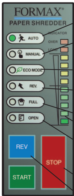
Control Panel
